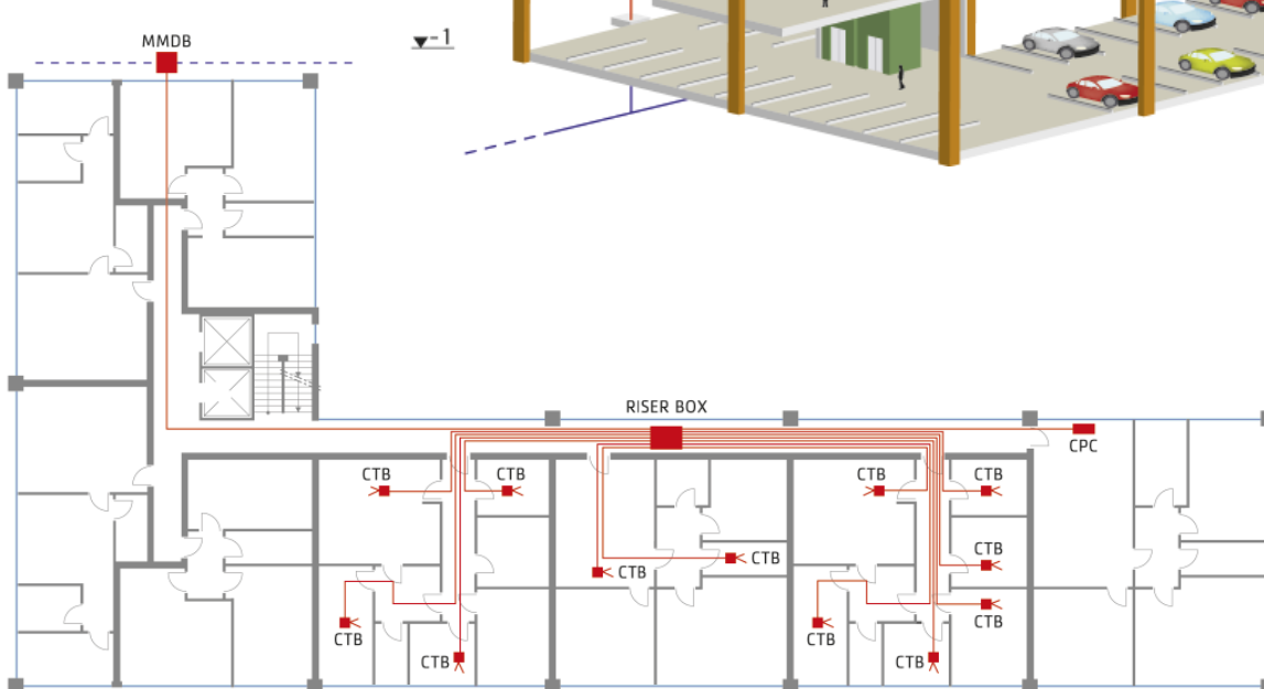
Floor 3
