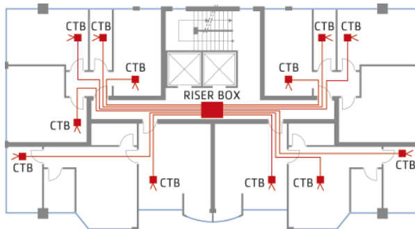
Floors 5 - 15 - 25
