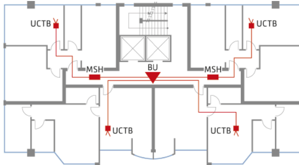
Floors 10 - 20 - 30
