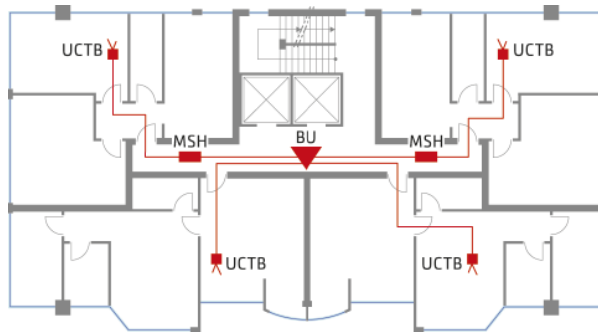
Floor 10
