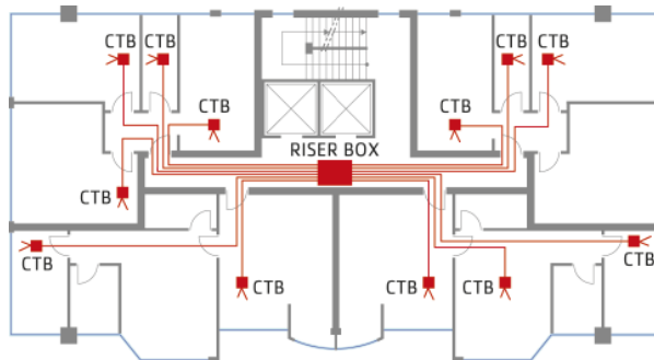
Floor 5
