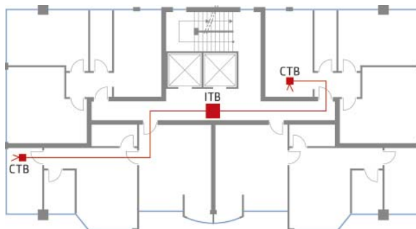
Floors 1 - 11 - 21
